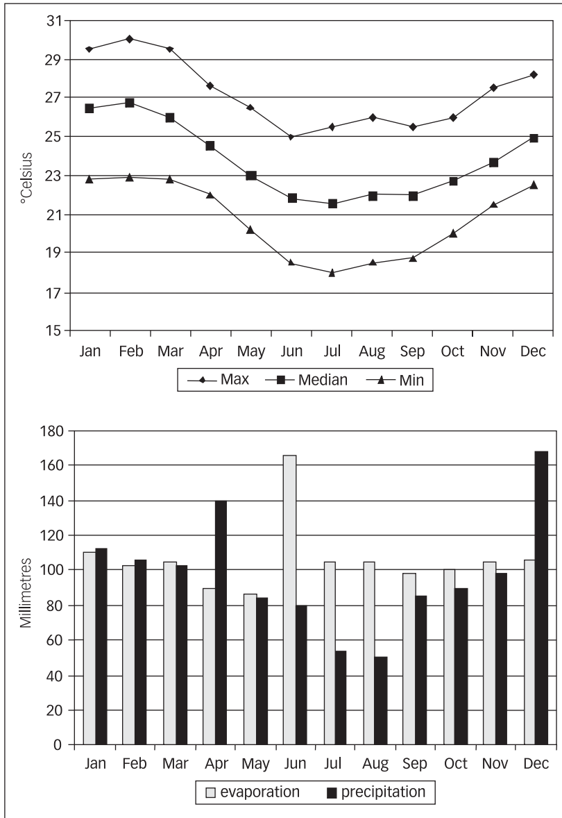
FIGURE 3 Average temperatures (top) and hydrographs (bottom) for Rio de Janeiro, 1961-1990
